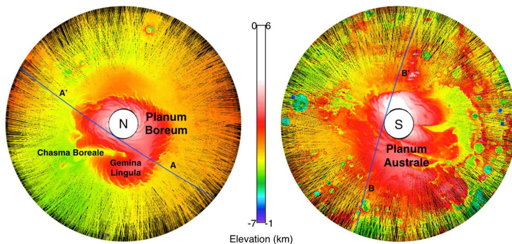
Figure 1. SHARAD ground track coverage (lines) colored by elevation above the Martian geoid (areoid) as computed using altimetry from Mars Orbiter Laser Altimeter (MOLA) across Planum Boreum (left) and Planum Australe (right). Elevation scales are offset between the north and south regions, the latter higher standing. Polar-projection maps extend to 69^\circ latitude in each hemisphere (2520 km diameter). Spacecraft orbits are offset from the pole, leaving a no-coverage zone poleward of \sim 87.4^\circ latitude. Blue lines are ground tracks corresponding to the radargrams shown in Figure 2.
