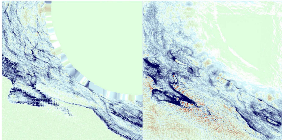
Figure 7. One of the 144 3-D interpolated and regularized (left) and 3-D downward continued (right) pieces from the Planum Boreum SHARAD 3-D volume overlapping the 3 rd quadrant of the coverage hole. Each such piece spans 237.5 km 2 . Color indicates radar return power (blue high, red low). As expected, the focusing performed by the downward continuation has significantly clarified the image, revealing previously blurred and/or obscured reflection features. Artifacts of the interpolation and regularization are visible inside the coverage hole, which get “smeared” by the downward continuation operator to create more artifacts inside the coverage hole.
