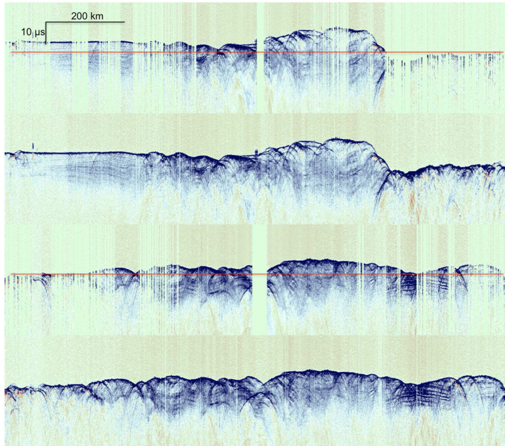
Figure 6. Inline (top pair) and crossline (bottom pair) profiles, transecting the Planum Australe 3-D volume just inside the polar coverage hole in map view, before (upper panel in pair) and after (lower panel in pair) 3-D interpolation and regularization. Color indicates radar return reflection strength (blue high, red low). Red lines on the profiles mark the location of the time slice shown in Figure 5. Comparison of the paired profiles shows that the coverage gaps across the ice caps have been mostly filled in by the interpolation and regularization.
