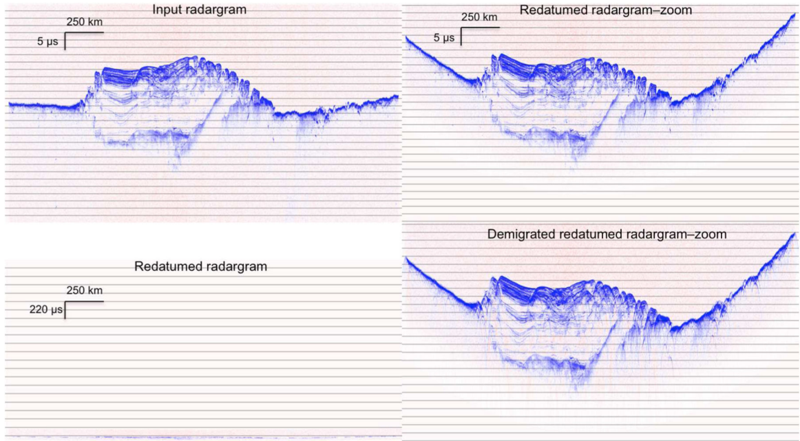
Figure 3. Results from the initial steps in the 2-D processing workflow used to prepare the radargrams for 3-D processing. The radargram from observation 11301-01 across Planum Boreum immediately after SAR processing (top left, vertical exaggeration 242:1), immediately after redatuming to the observation’s original orbit datum (bottom left, vertical exaggeration 7:1 and top right, vertical exaggeration 272:1), and immediately after demigration at at this same datum (bottom right, vertical exaggeration 272:1). Color indicates radar return power (blue high, red low). After redatuming the input radargram back to its orbit datum, the radar returns are barely visible at the bottom of the lower left panel (even with a 7:1 vertical exaggeration). Scrutinizing and comparing the two right panels, the range migration focusing has been removed by the demigration as desired.
