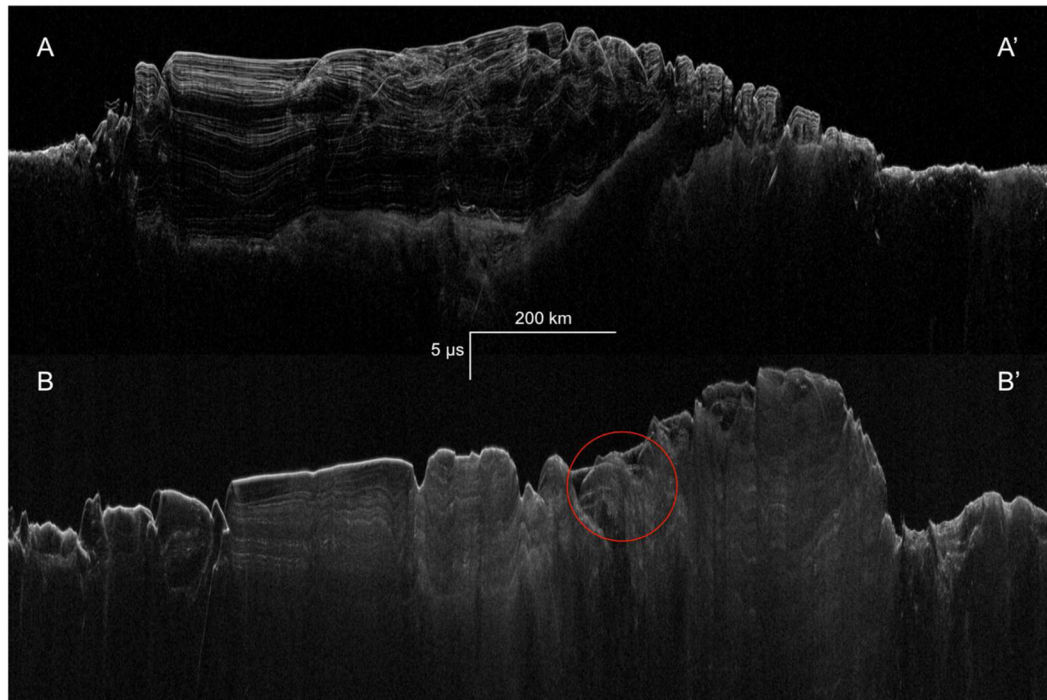
Figure 2. Segments of Planum Boreum SHARAD radargram from observation 11301–01 (top) and Planum Australe SHARAD radargram from observation 27199–01 (bottom) after pre-processing. Grayscale represents radar return power (light high, dark low). The differences in the reflectivity character evident between these two radargrams are typical throughout the two polar ice caps. The feature circled in red, and partially obscured by discordant radar returns (“clutter”), is one of the CO 2 ice deposits characterized by so-called “reflection free zones” (RFZs) separated by distinct reflectors thought to be water ice.
