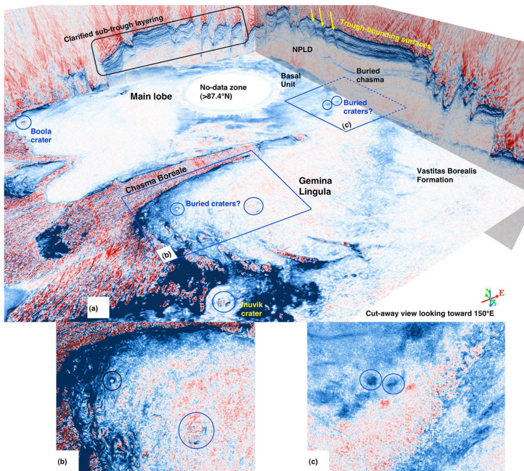
Figure 12. Cut-away views into the depth-converted 3-D volume of SHARAD data, showing radar return power (blue high, red low) from features within Planum Boreum. (a) Perspective view encompassing all of Planum Boreum. For scale, the no-data zone is 310 km across and the stack of NPLD layers to the right of the buried chasma is 2 km thick. Labeled features are discussed in the text. (b, c) Zoomed-in views with enhanced contrast at the constant-depth slice in (a), showing possible buried craters within the circles.
