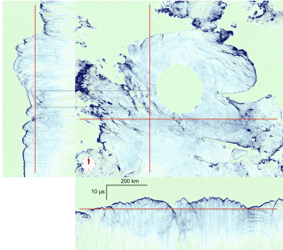
Figure 10. Inline profile (upper left), time slice (upper right), and crossline profile (lower right) through the Planum Australe SHARAD 3-D volume before 3-D downward continuation. Color indicates radar return reflection strength (blue high, red low). Thin red lines mark locations of adjacent views. Surface and subsurface radar returns are unfocused, leaving structure unresolved and an image “cluttered” by these unfocused returns. In particular, a feature (bracketed by the two thin dashed lines on the inline and time slice panels) characterized by so-called “reflection free zones” (RFZs) separated by distinct bright reflectors is mostly obscured by clutter prior to downward continuation (compare with Figure 11). This same feature appears in the near-by radargram segment from observation 27199–01 shown in the bottom panel of Figure 2.
