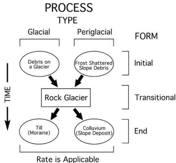
Figure 13. Diagram illustrating the alpine landscape continuum (modified from Giardino and Vitek [1988b]). Rock glaciers are transitional forms that can develop from two distinct processes and can progress to two distinct end-members. Rate of movement is related to process, not form.
